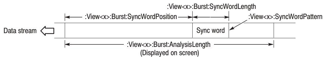
Figure 4–12: Setting the GSM measurement parameters
